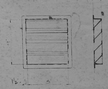
TYP. VENT LOUVE 2-REQD - BACK SAME DETAILS AS LOUVER DWG M-313
