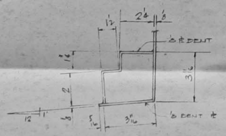
SECTION 6-6
