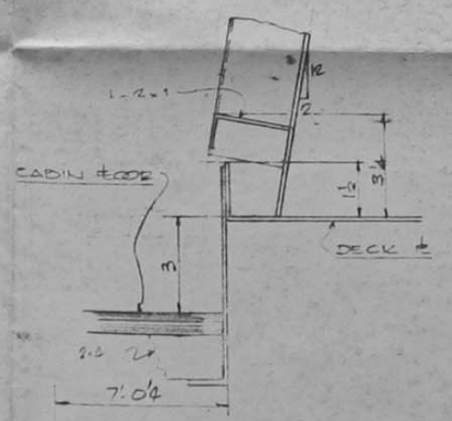
SECTION 9-9
