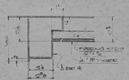
SECTION 12-12
