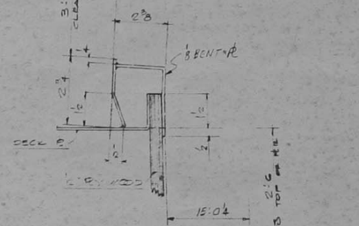
SECTION 10-10 AT CENTRE LINE
