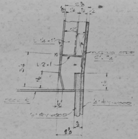
SECTION 3-3
